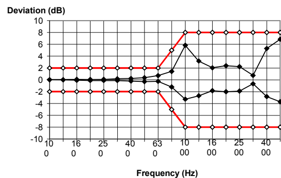
Directivity in accordance with ISO 3382
