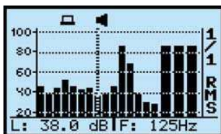
1/1 octave analysis
