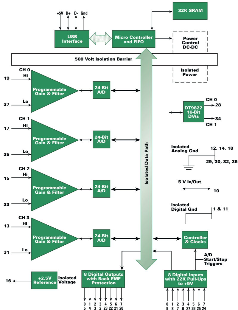
DT9821-22 Block Diagram
