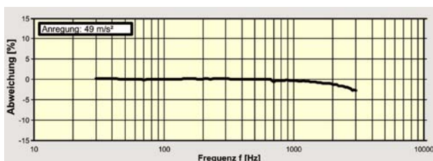
Frequency response Model 102M/CM
